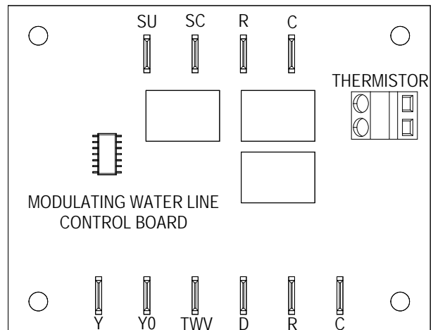
FIGURE 27 Modulating Water Line Control
