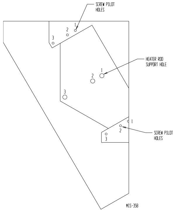
FIGURE 3 Screw Mounting Holes
