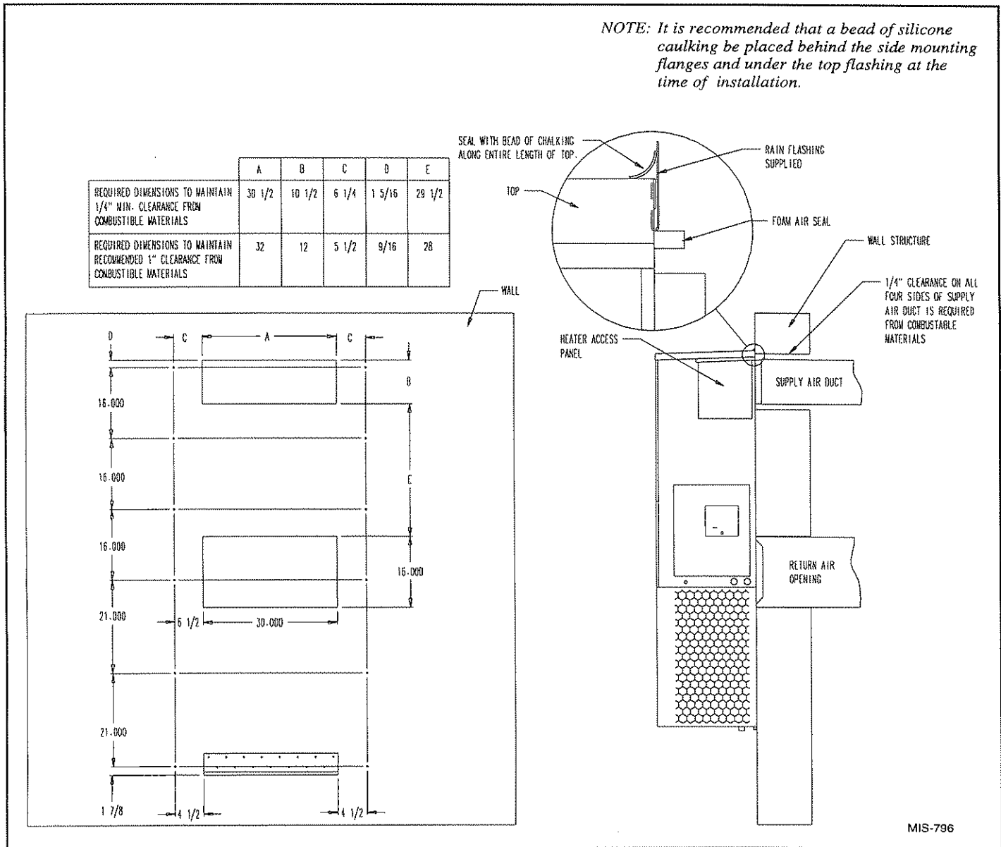
FIGURE 3 MOUNTING INSTRUCTIONS
