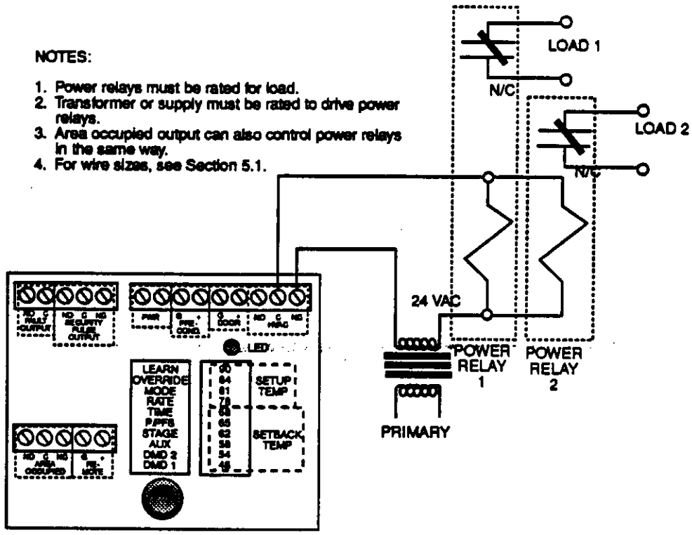
Figure B1 Typical Power Relay Wiring Diagram. External Relays Can Be Controlled from CS 's HVAC or Auxiliary Relays.
