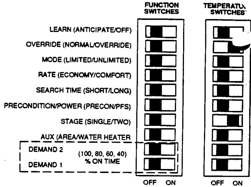
Figure 1 CS 2000 Function Switches.
