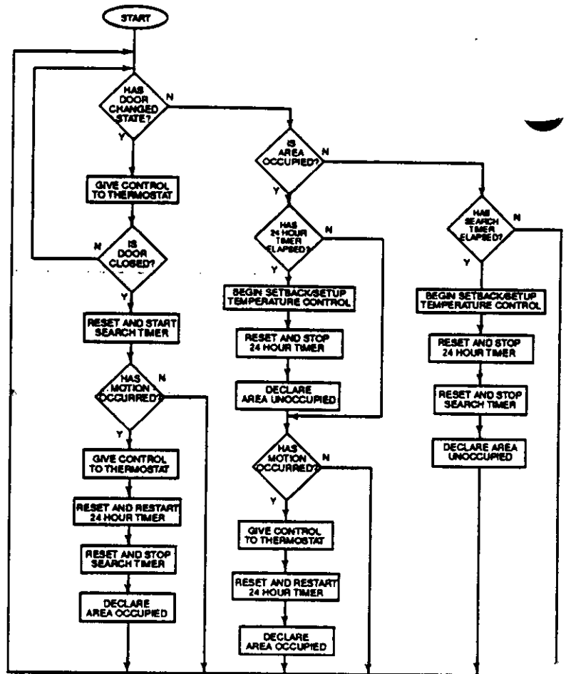
Figure 3 Simplified Flow Chart for CS 2000's Limited Access Mode. (24-hour occupancy recheck also shown.)
