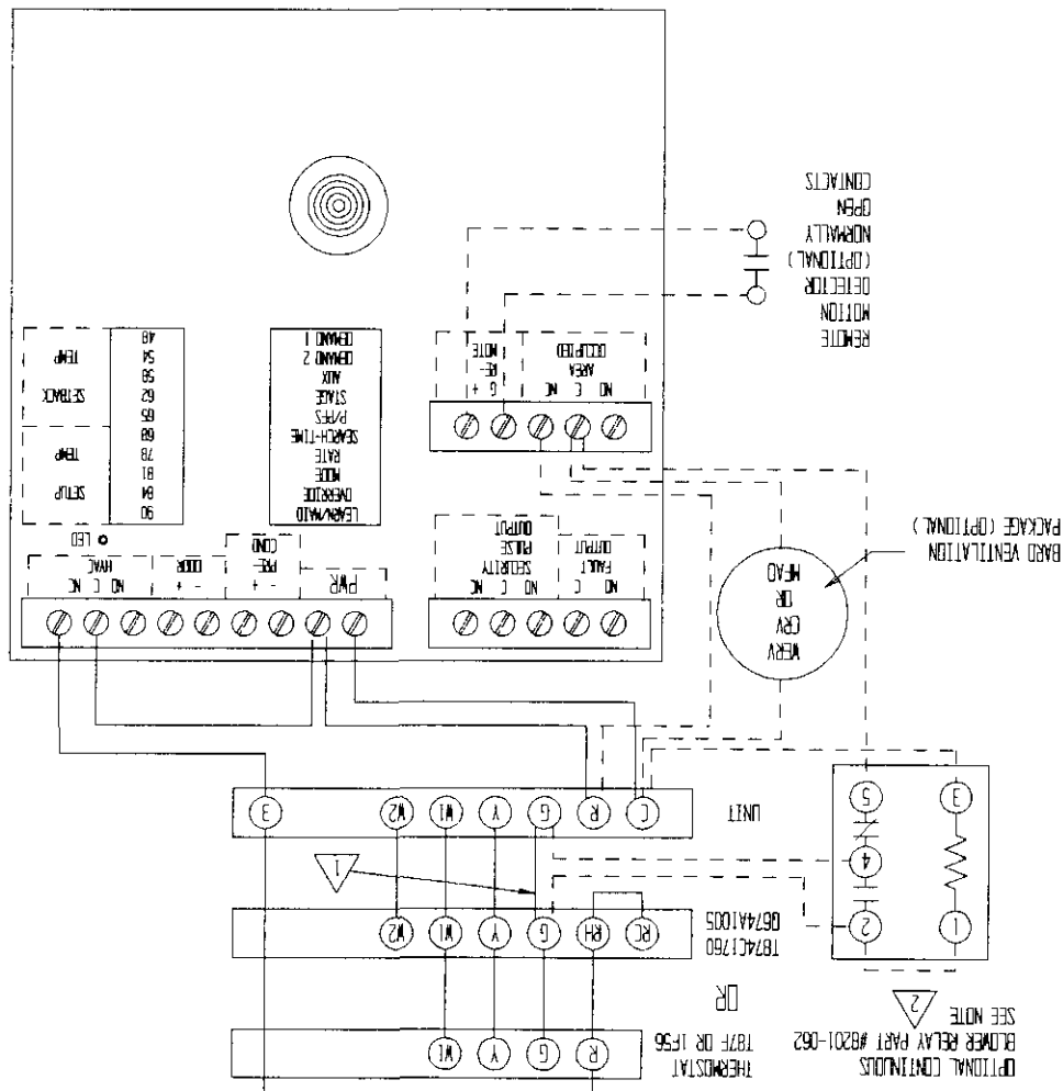
AIR CONDITIONER CONNECTION DIAGRAM
