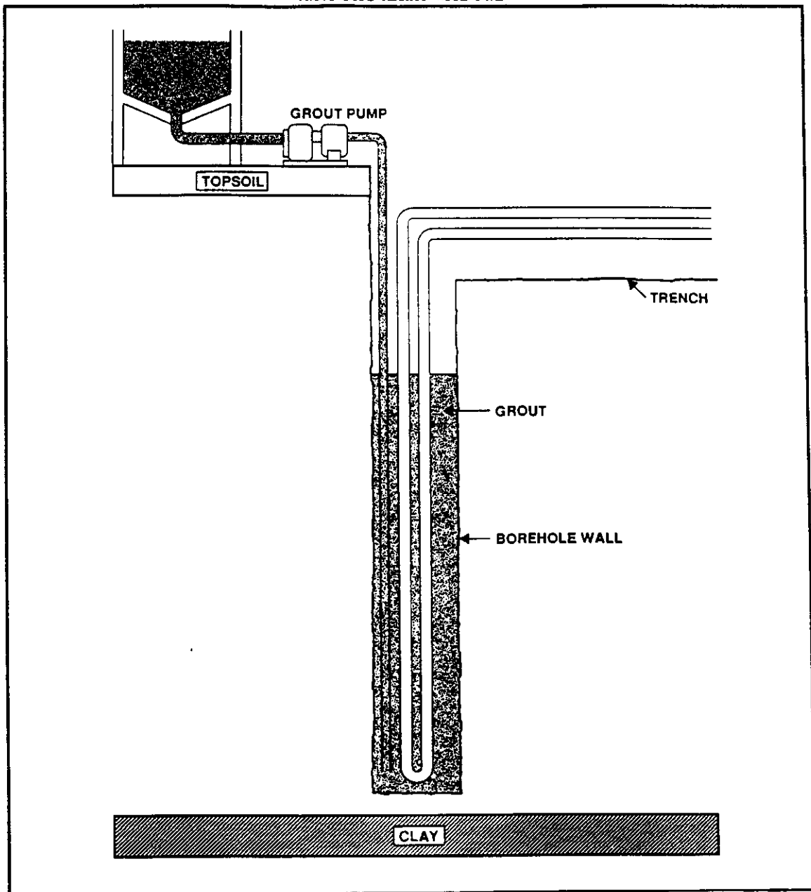
FIGURE 22A GROUT PIPE METHOD WITH PUMP
