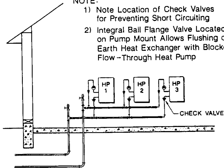
FIGURE 30 MULTIPLE UNIT INSTALLATION
