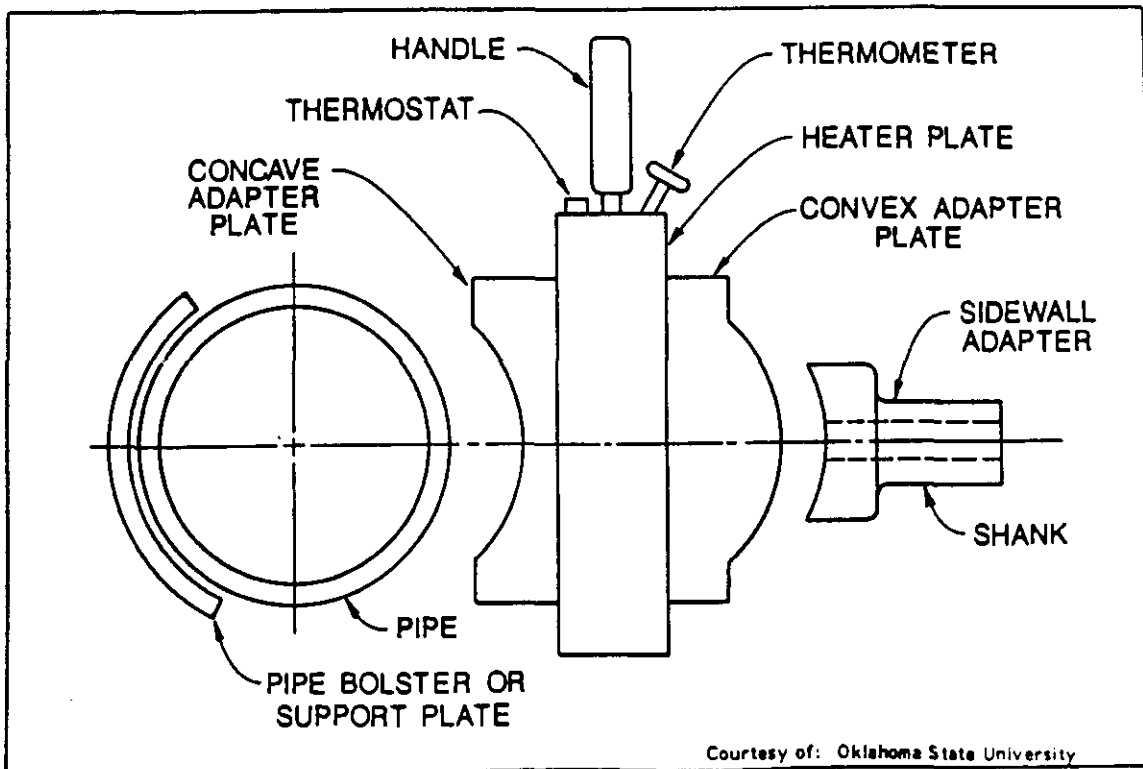
FIGURE 17 SIDEWALL FUSION
