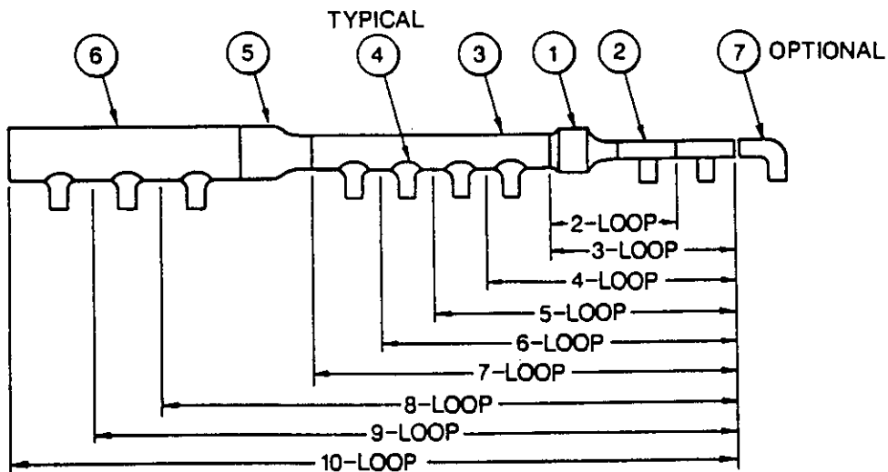
FIGURE 31B TEN-TON HEADER SYSTEM--PB PIPE--BUTT FUSED
