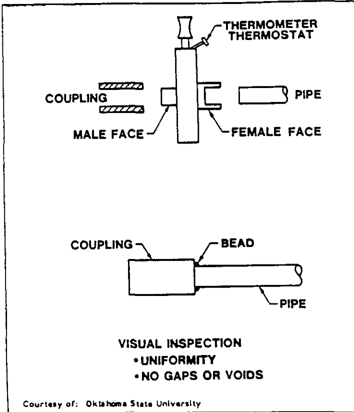
FIGURE 15 SOCKET FUSION
