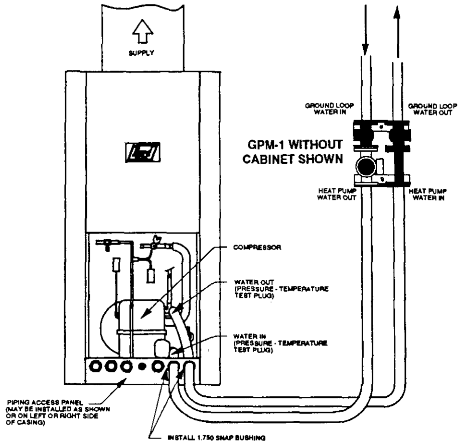
FIGURE 27 PUMP MODULE HOOKUP
