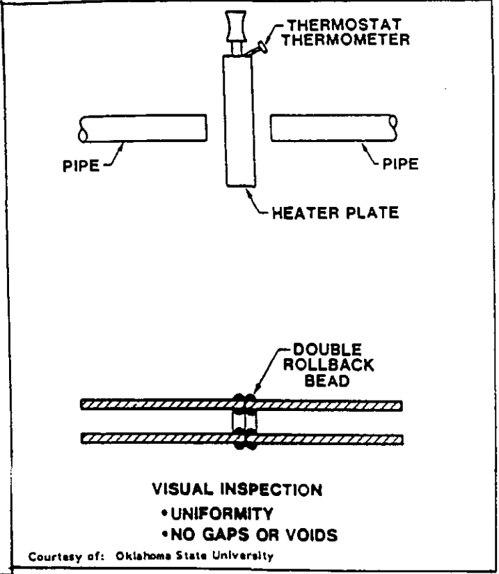
FIGURE 16 BUTT FUSION
