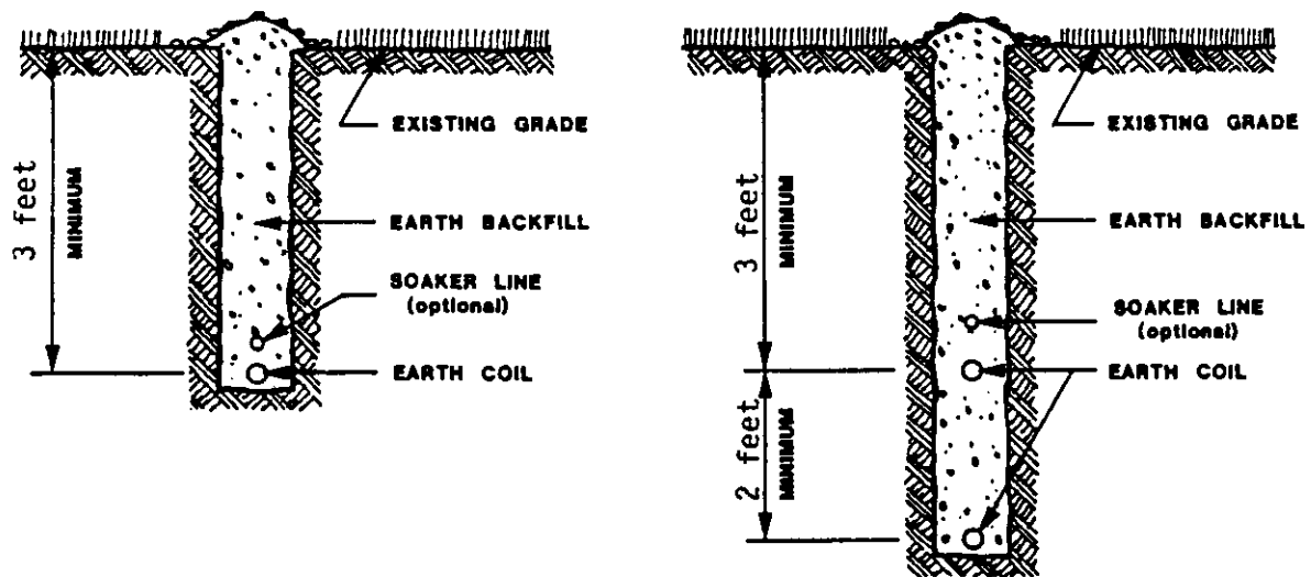
FIGURE 5 SINGLE AND STACKED HORIZONTAL EARTH COILS
