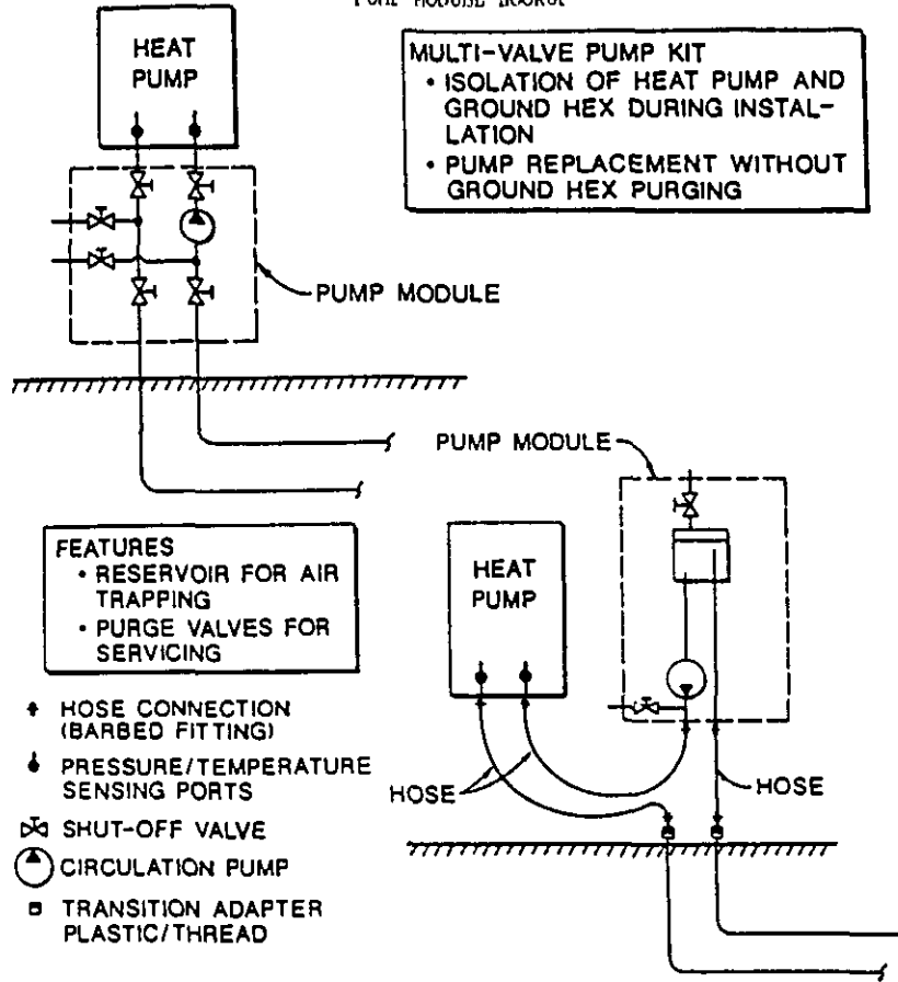
FIGURE 27 PUMP MODULE BACKUP
