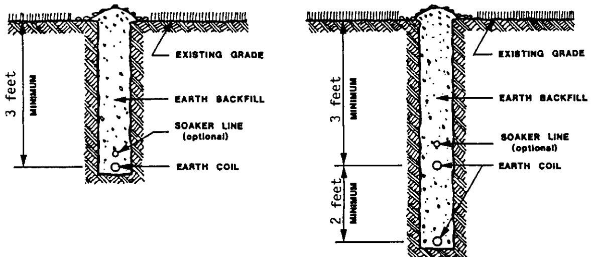
FIGURE 5 SINGLE AND STACKED HORIZONTAL EARTH COILS
