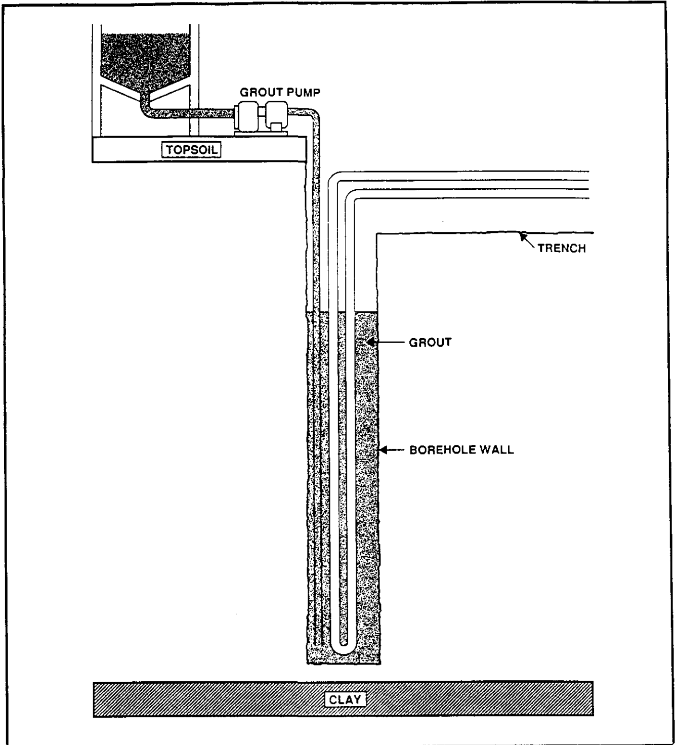
FIGURE 22A GROUT PIPE METHOD WITH PUMP
