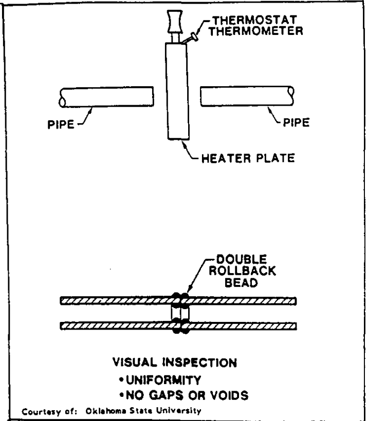
FIGURE 16 BUTT FUSION
