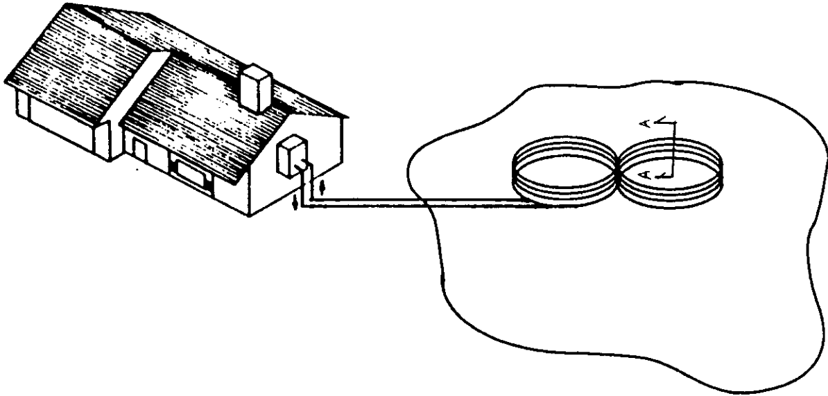
FIGURE 34 VERTICAL SYSTEM POND LOOP SYSTEM
