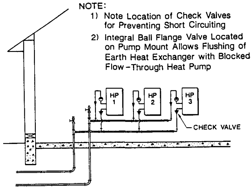
FIGURE 29 LAYOUT AND DETAILS OF A TYPICAL CL/GS HEAT PUMP SYSTEM
