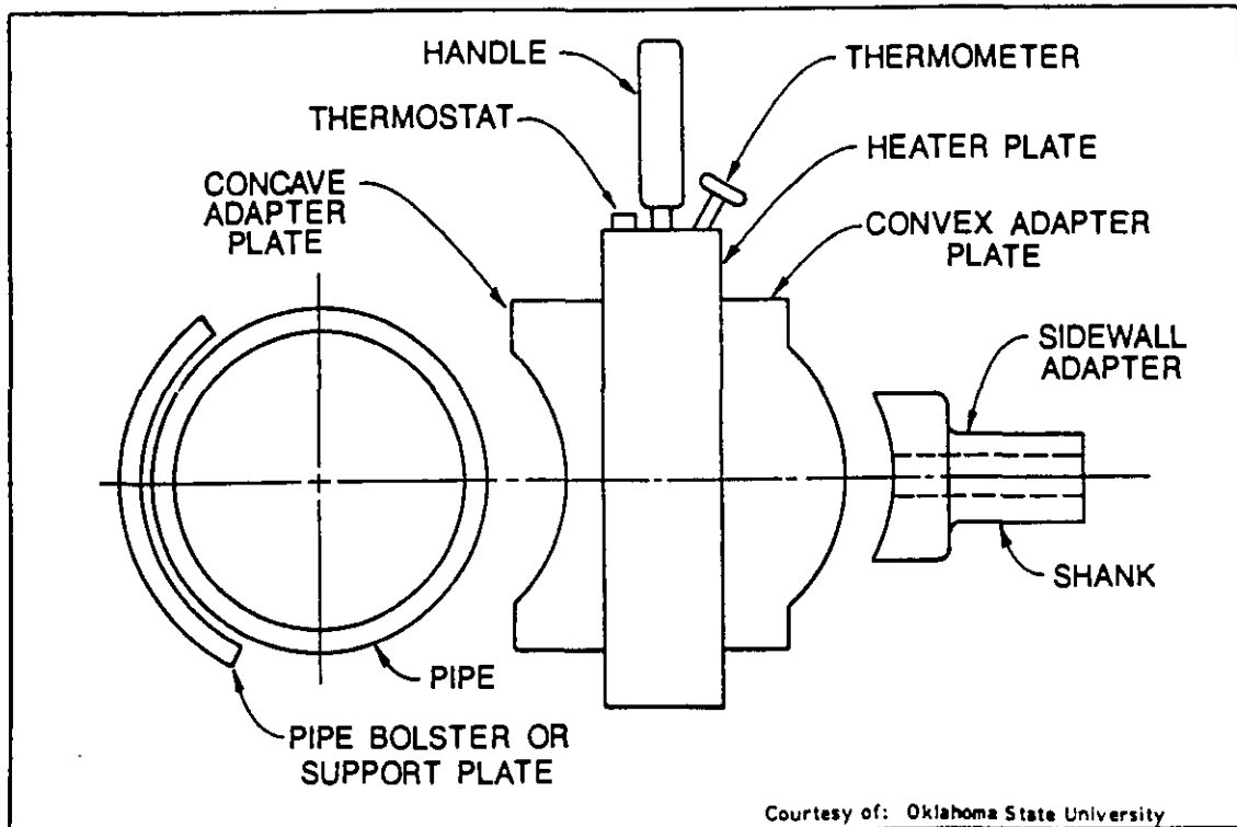
FIGURE 17 SIDEWALL FUSION
