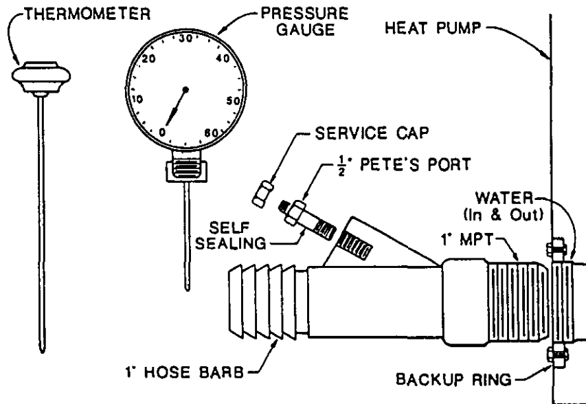
FIGURE 28 PRESSURE AND TEMPERATURE SENSING ADAPTER AND COMPONENTS
