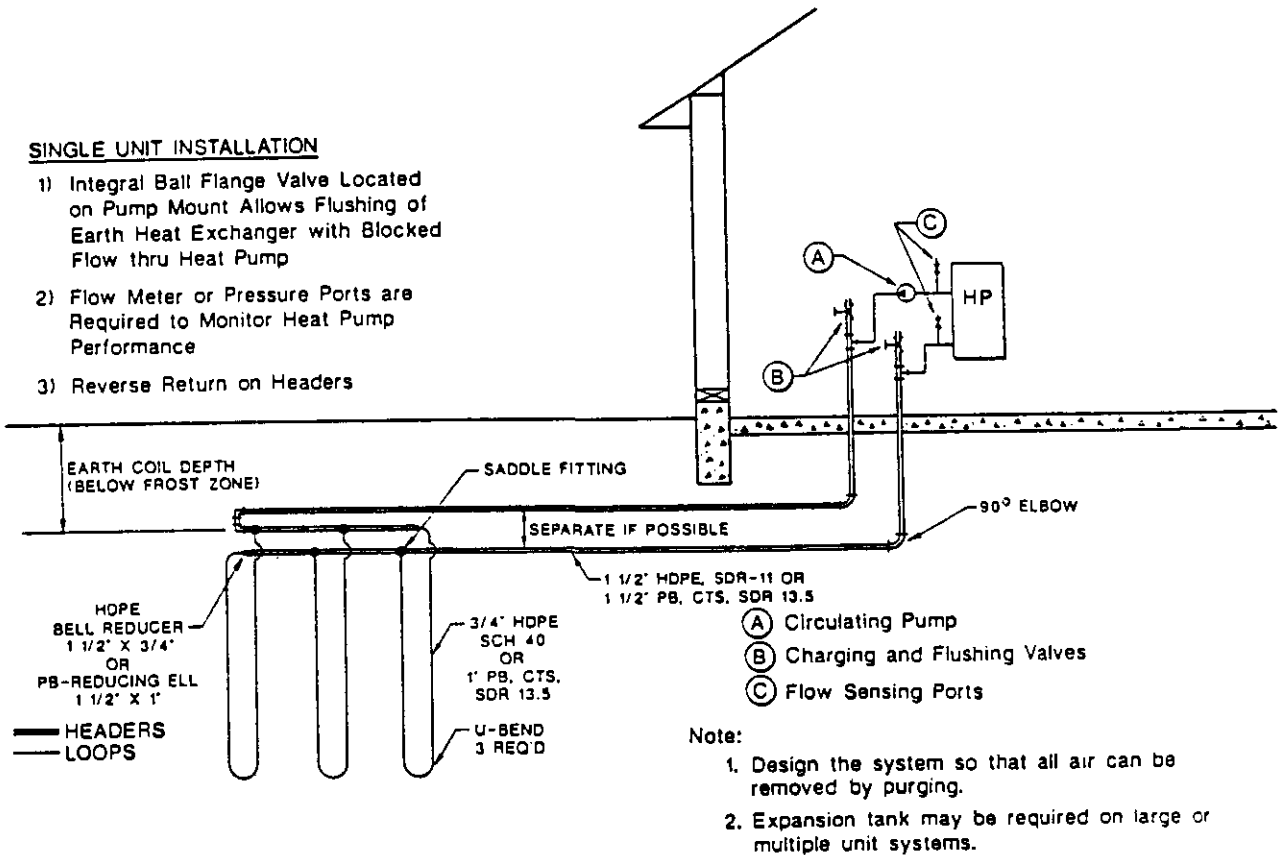
FIGURE 30 MULTIPLE UNIT INSTALLATION
