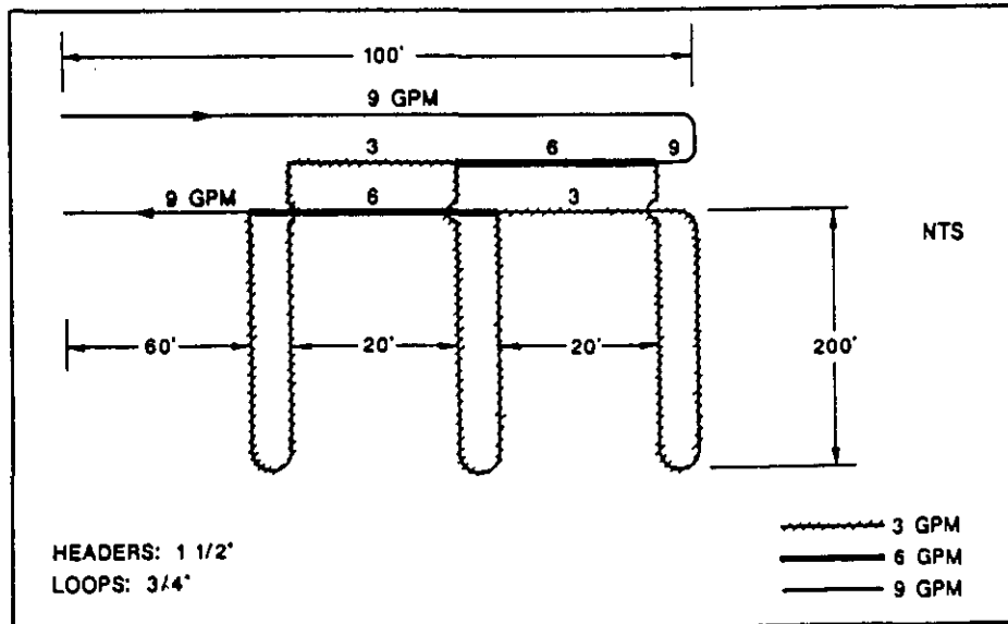
FIGURE 10C SPACED HEADER WITH REVERSE RETURN
