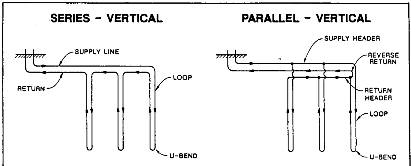
FIGURE 3A SERIES AND PARALLEL VERTICAL SYSTEMS
