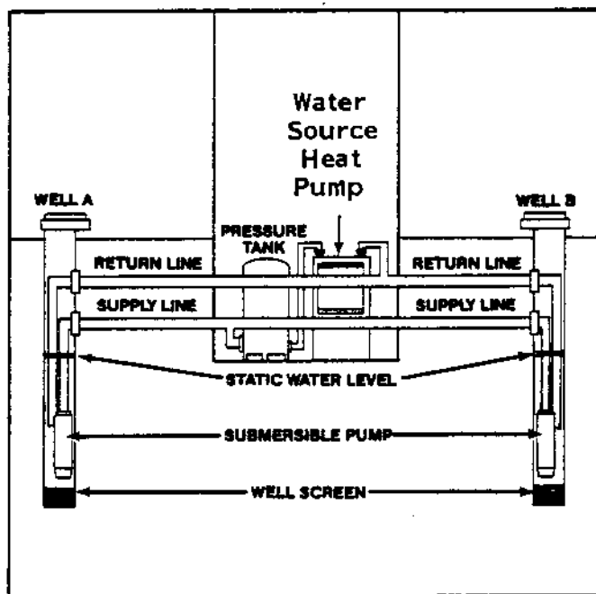
Figure 5. TWO WELL REVERSIBLE SYSTEM
