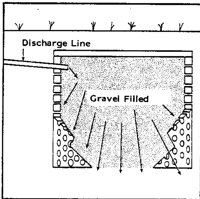
Figure 2. DRY WELL
