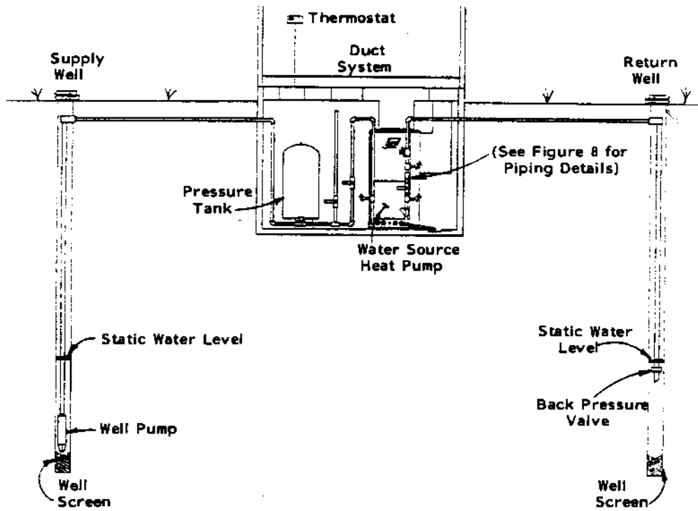
Figure 9. TYPICAL RETURN WELL SYSTEM
