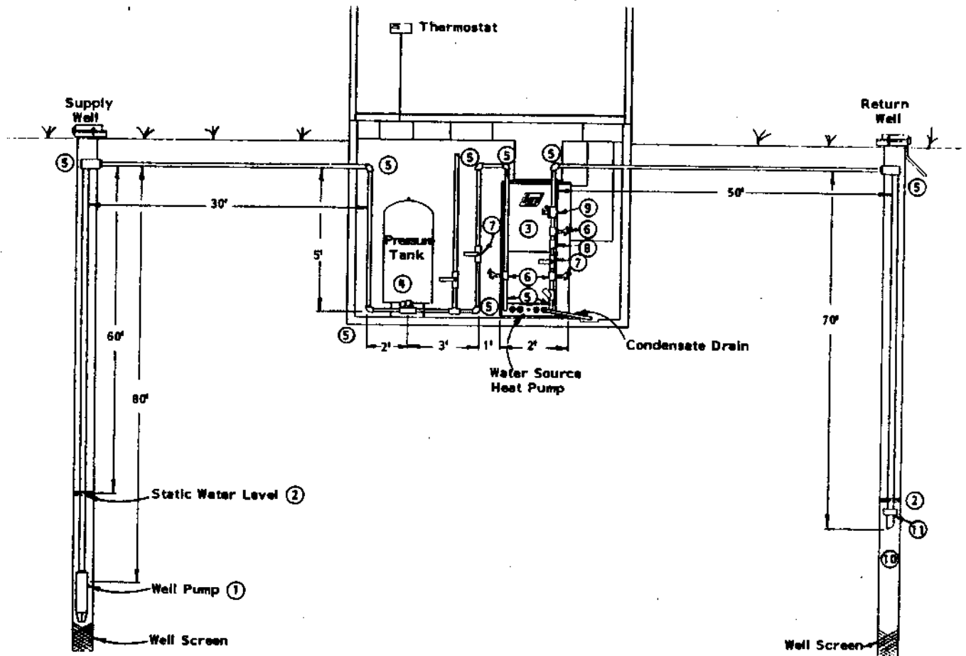
Figure 7. TYPICAL RETURN WELL SYSTEM
