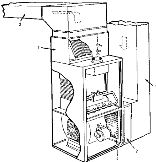
Illustration of accumulated pressure drop through ducts & accessories.
