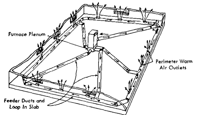
Figure 1. The perimeter loop system is particularly effective in colder climates. It has excellent utility in houses built on slabs in that good heat distribution is insured and floors are kept warm also.
