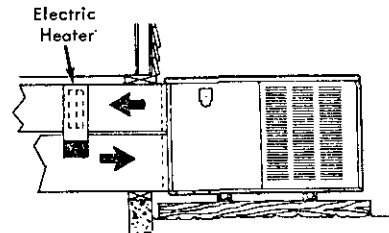
Typical self-contained air conditioner or heat pump installed in a through-the-wall manner.
