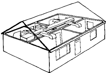
Overhead Attic Supply Ductwork with Ceiling Diffusers
