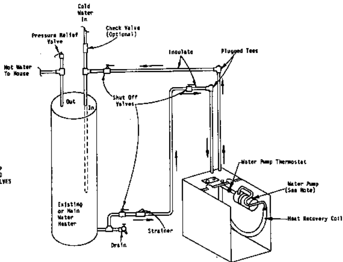
TYPICAL "WQSD" MODEL ONE TANK INSTALLATION (PERMISSIBLE)
