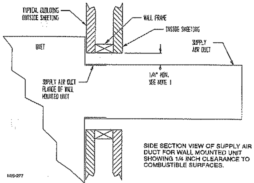
FIGURE 4 ELECTRIC HEAT CLEARANCE
