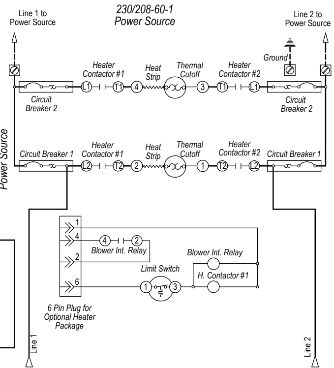
Ladder Diagram
