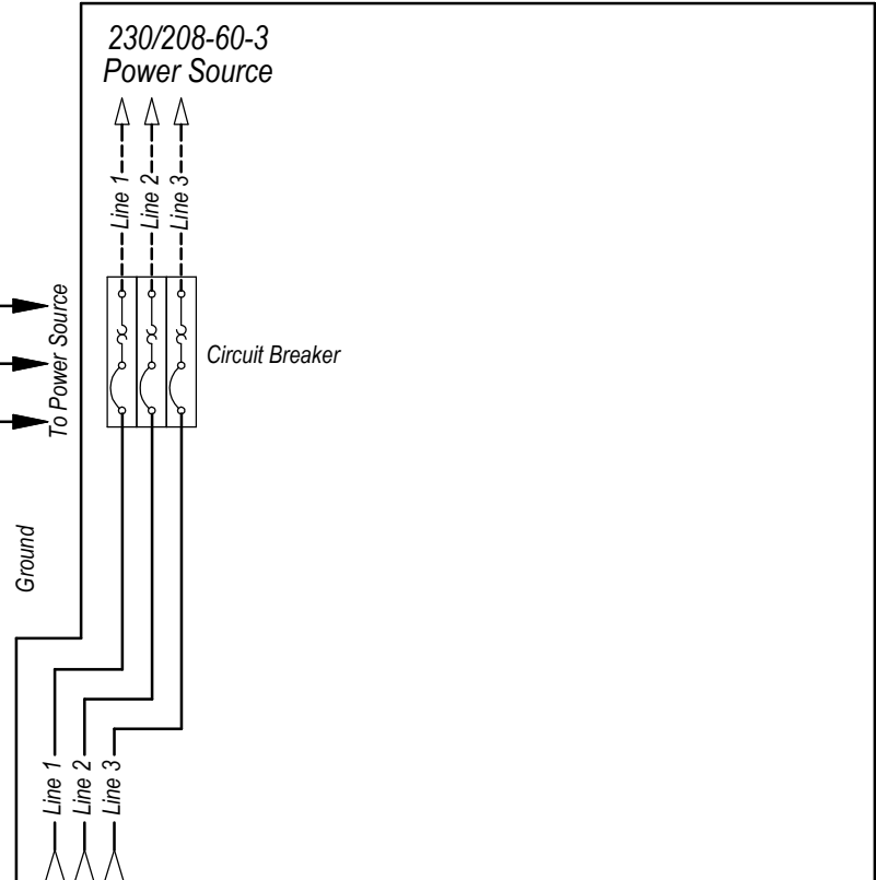
Ladder Diagram
