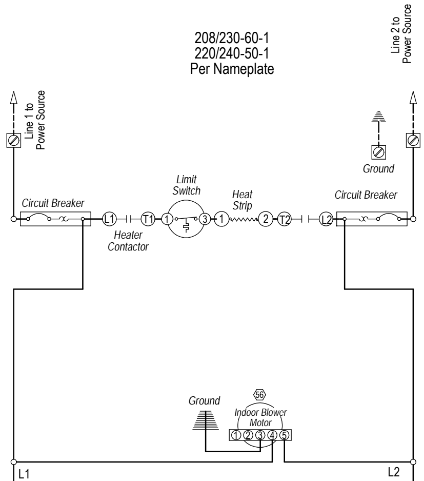
Ladder Diagram
