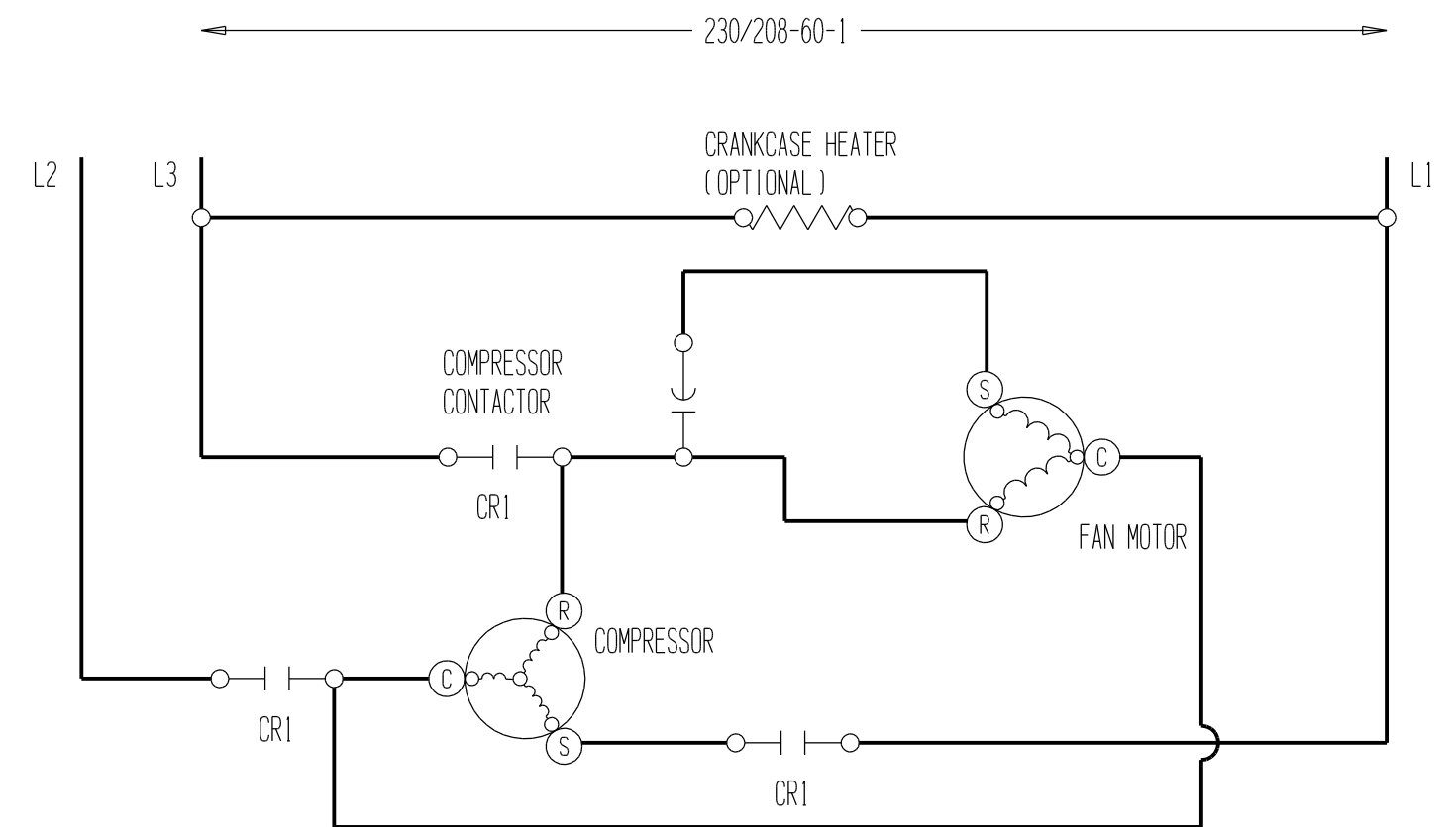
HIGH VOLTAGE CIRCUIT
