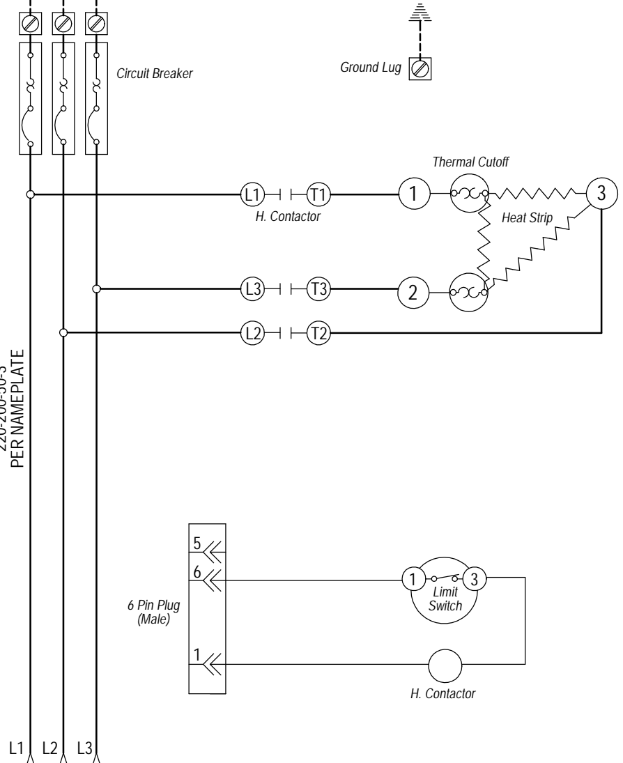
Ladder Diagram
