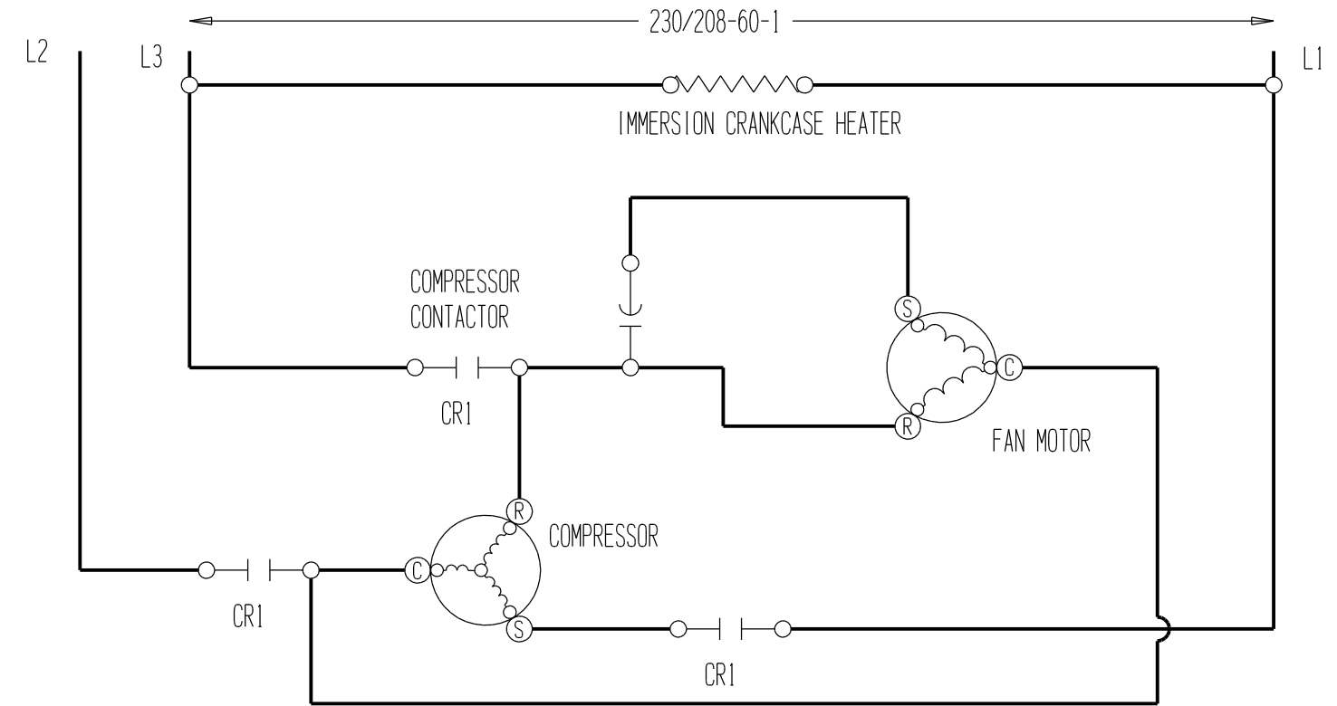
HIGH VOLTAGE CIRCUIT
