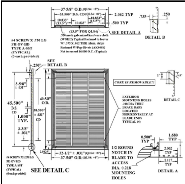
An attractive mechanical air louver with a removable service core that utilizes our exclusive shading "C" blade.
