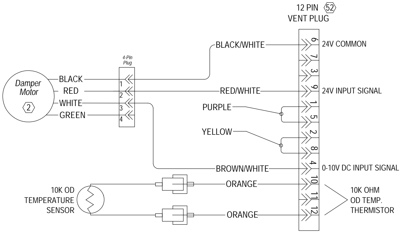
NO CONTROL ECONOMIZER WIRING DIAGRAM
